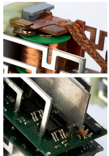
Mechanical original glow plug relay (top) vs. intelligent semiconductors in the Hitachi No. 2502183 (below)
