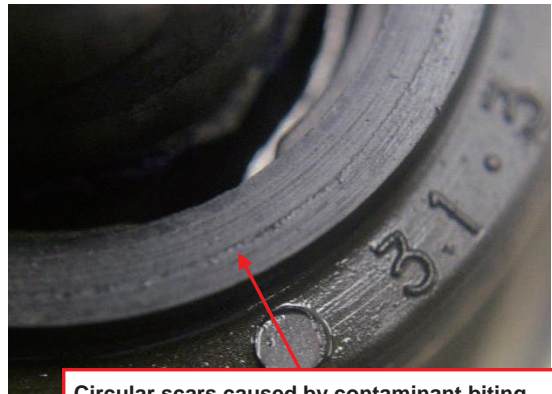
Contaminant biting
