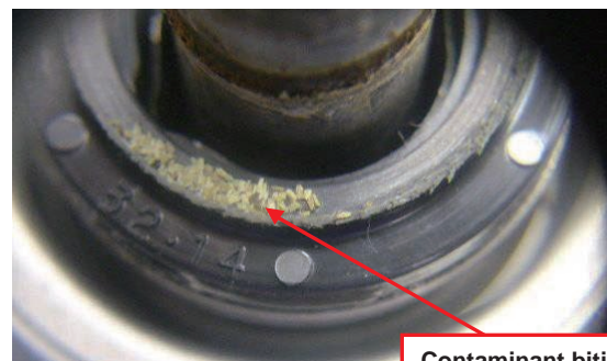
Contaminant biting
